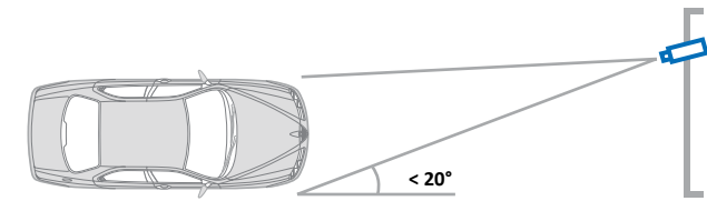
CAMERA ANGLE NO GREATER THAN 20 DEGREES FOR SIDE MOUNT INSTALLATIONS
