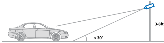
THE CAMERA SHOULD BE MOUNTED AT AN ANGLE NO GREATER THAN 30 DEGREES
